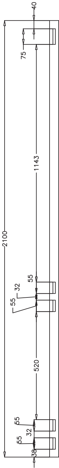
LEFT AND RIGHT STILE WINDSOR HERITAGE 90 X 210
